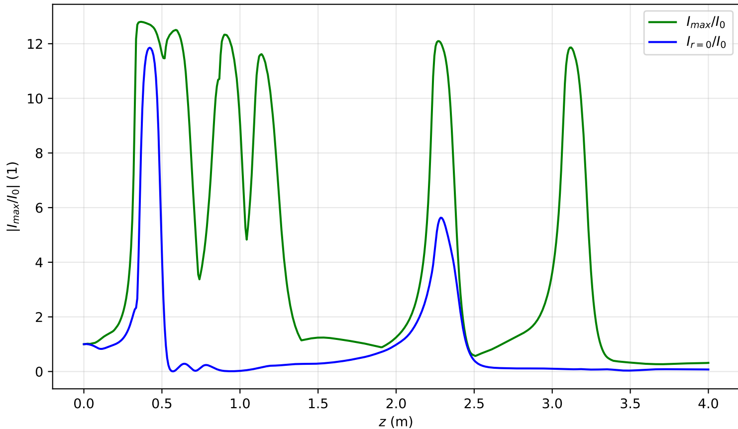
I_{max}(x = 0, y = 0, z)/I_0 , P_{in}=8.7P_{cr} , noisy input, artificial time
